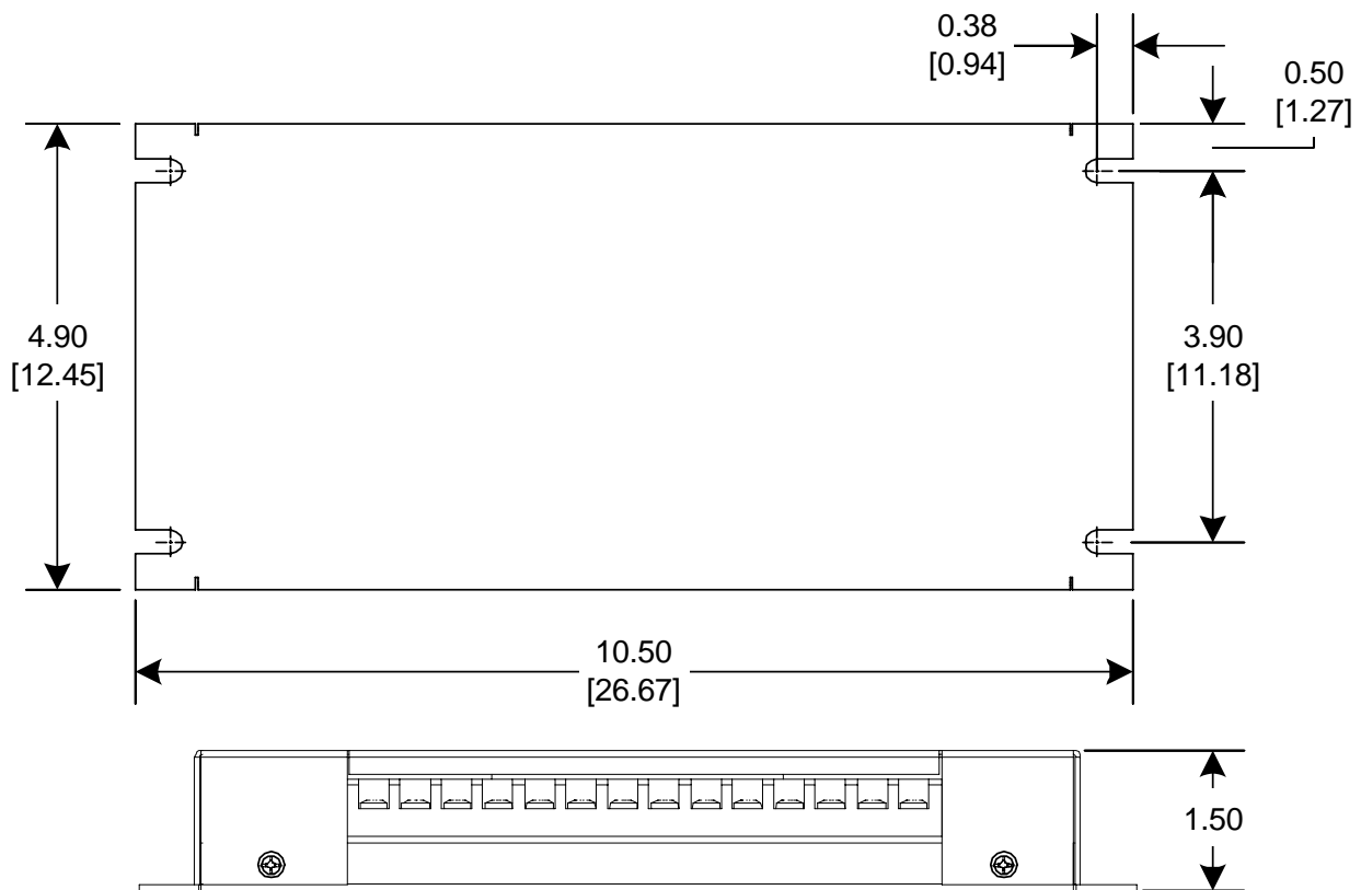
Figure 2 Universal Contact Input Adapter
